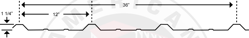
PBR Panel Diagram
